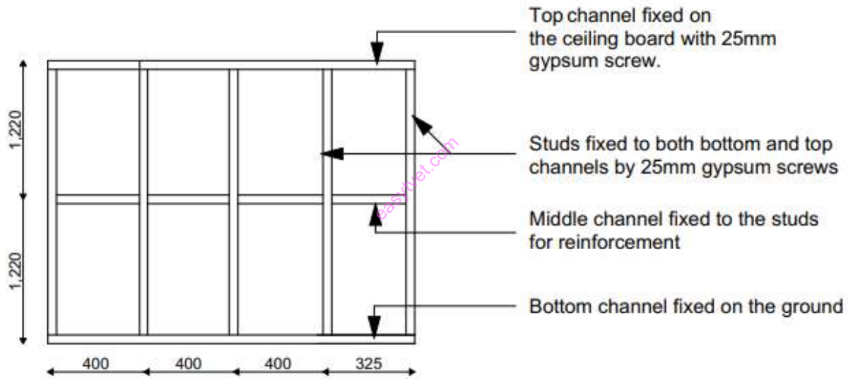
SECTION B-B ; Framed structure
