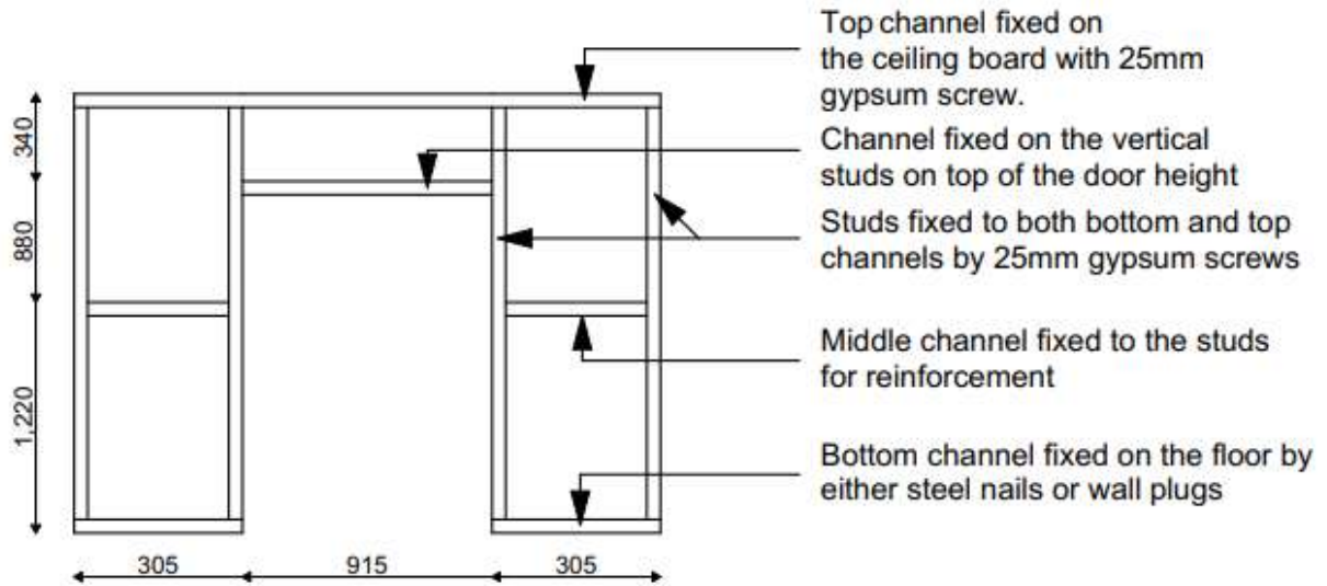
SECTION A-A ; Framed structure
