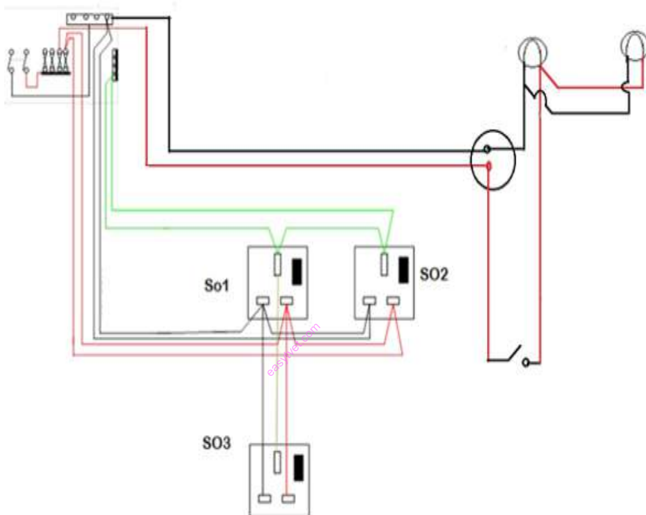
Figure 1: Wiring Diagram
